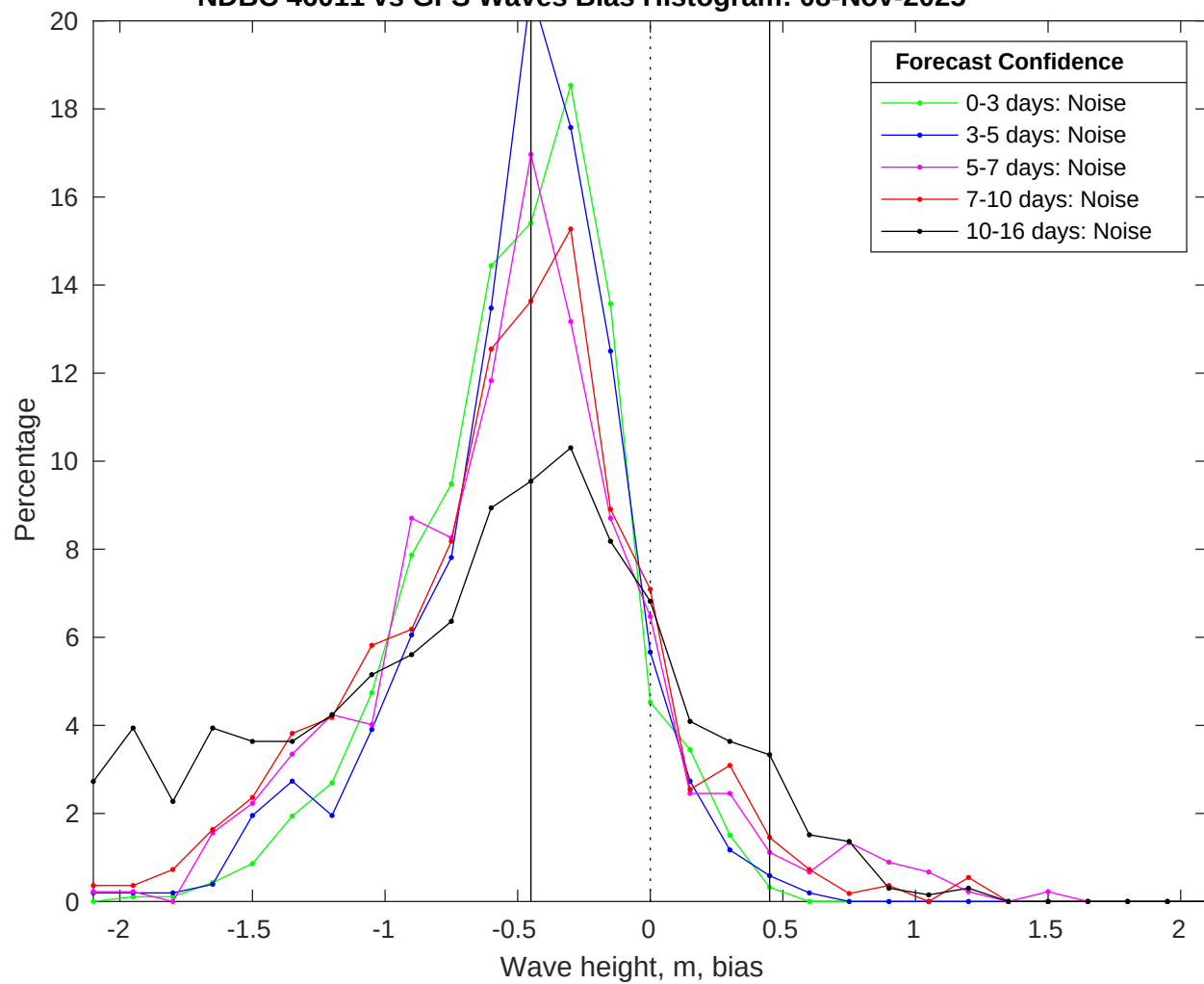
NDBC 46011 vs GFS Waves Bias Histogram: 08-Nov-2025
