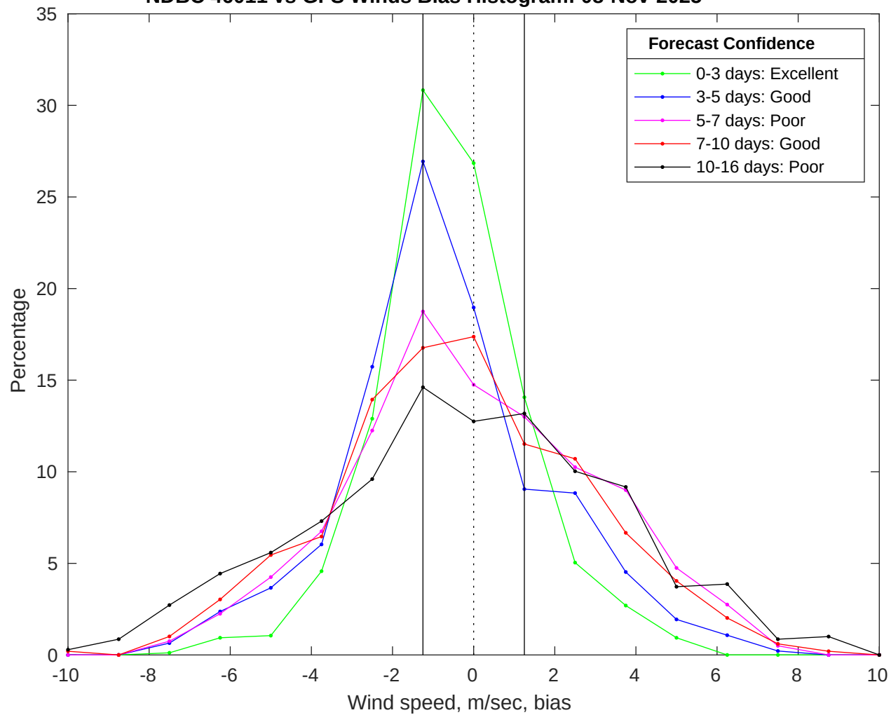
NDBC 46011 vs GFS Winds Bias Histogram: 08-Nov-2025
