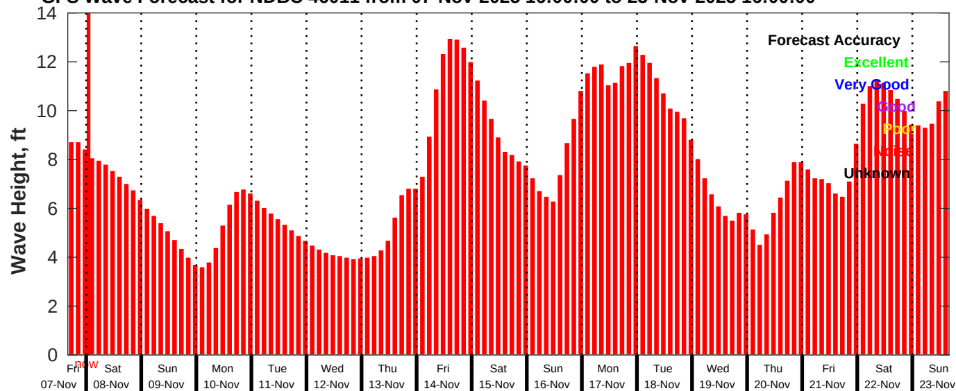
GFS Wave Forecast for NDBC 46011 from 07-Nov-2025 16:00:00 to 23-Nov-2025 16:00:00
