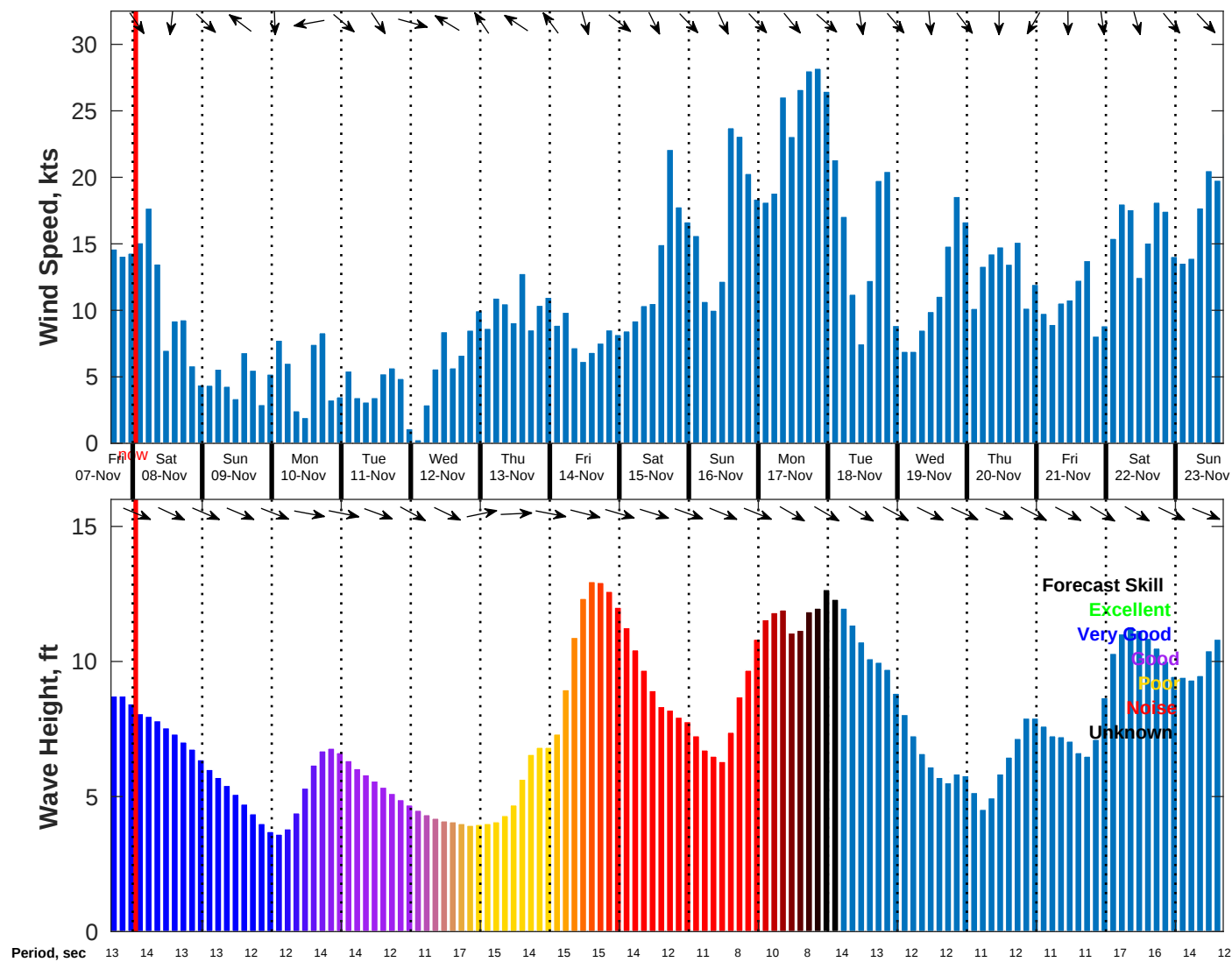
Wind & Wave Forecast for NDBC 46011 from 07-Nov-2025 16:00:00 to 23-Nov-2025 16:00:00
