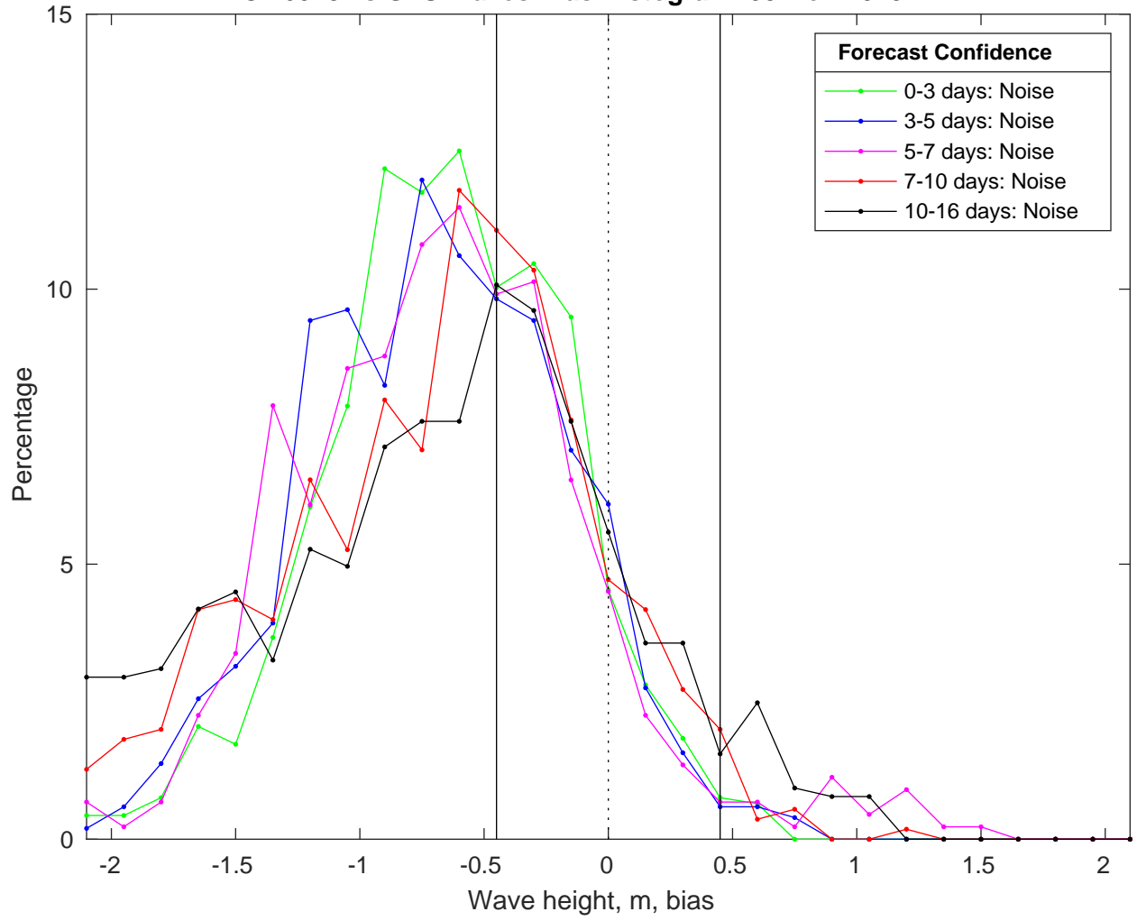
NDBC 46028 vs GFS Waves Bias Histogram: 08-Nov-2025
