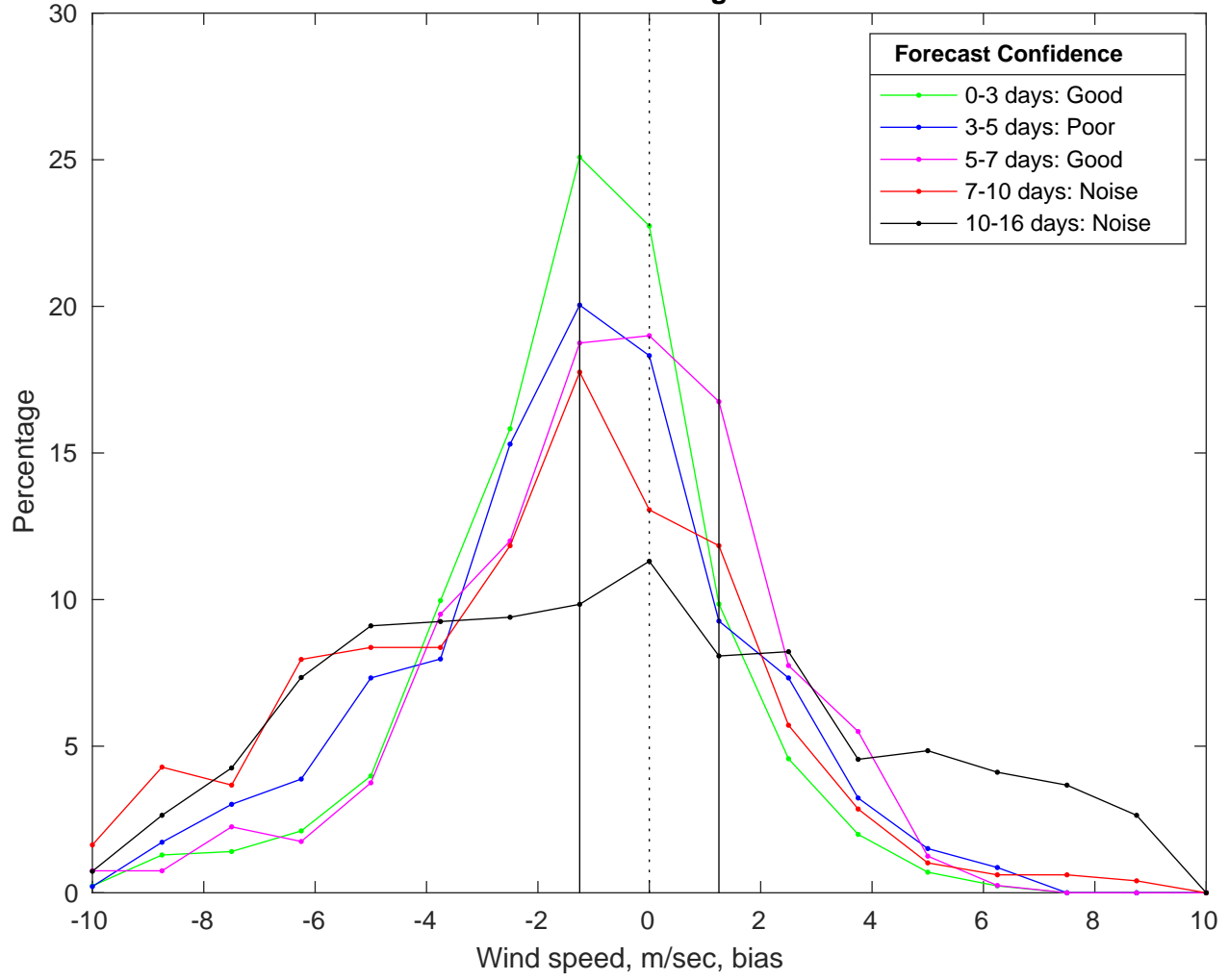
NDBC 46054 vs GFS Winds Bias Histogram: 08-Nov-2025
