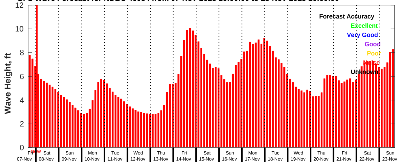
GFS Wave Forecast for NDBC 46054 from 07-Nov-2025 16:00:00 to 23-Nov-2025 16:00:00
