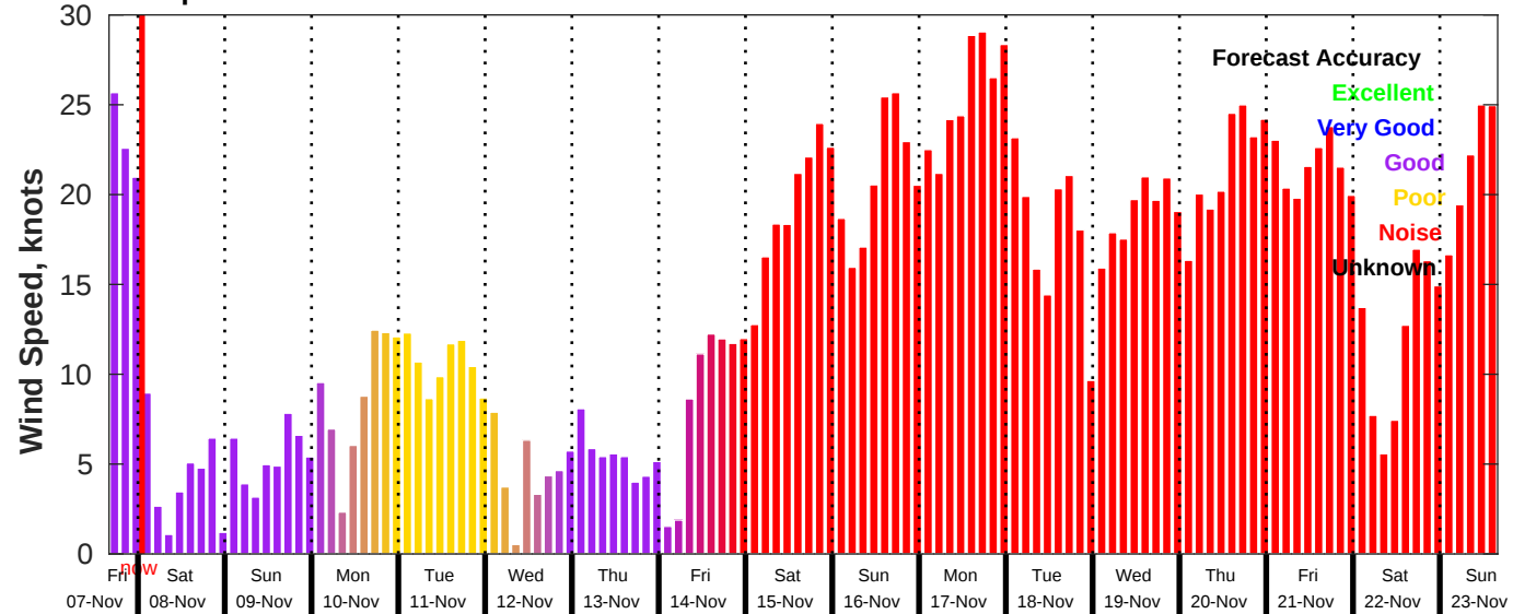
GFS Wind Speed Forecast for NDBC 46054 from 07-Nov-2025 16:00:00 to 23-Nov-2025 16:00:00
