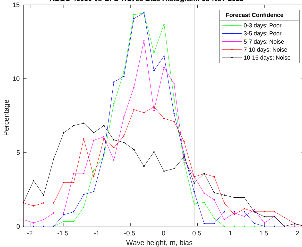
NDBC 46059 vs GFS Waves Bias Histogram: 08-Nov-2025
