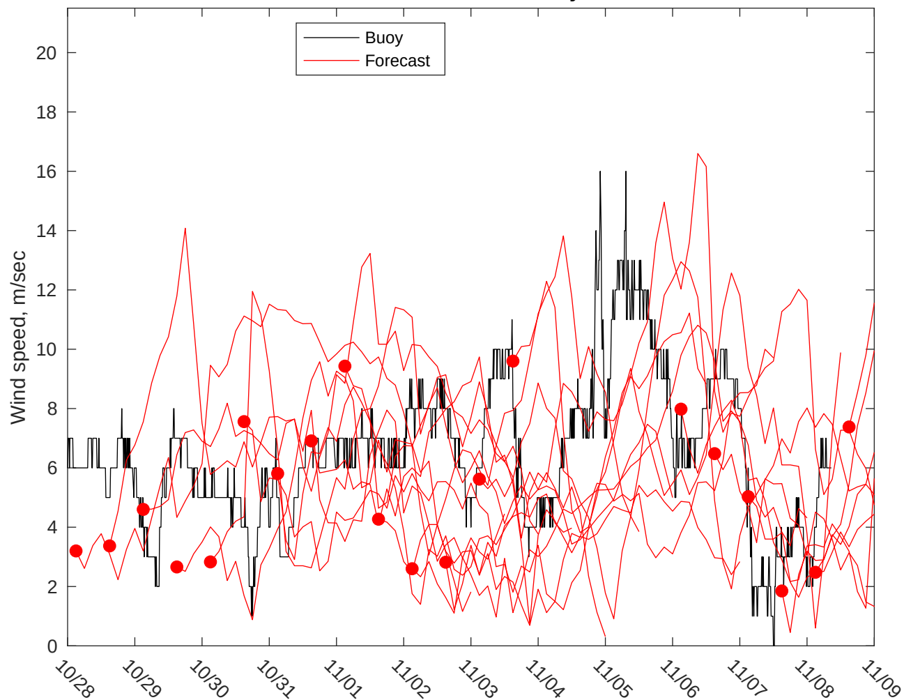
NDBC 46059 vs GFS Winds: 10 to 16 day forecast
