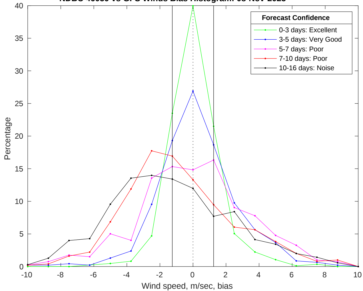
NDBC 46059 vs GFS Winds Bias Histogram: 08-Nov-2025
