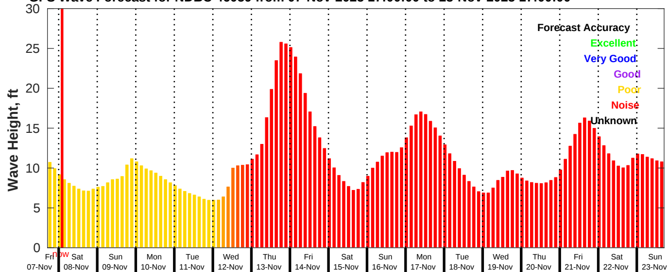
GFS Wave Forecast for NDBC 46059 from 07-Nov-2025 17:00:00 to 23-Nov-2025 17:00:00
