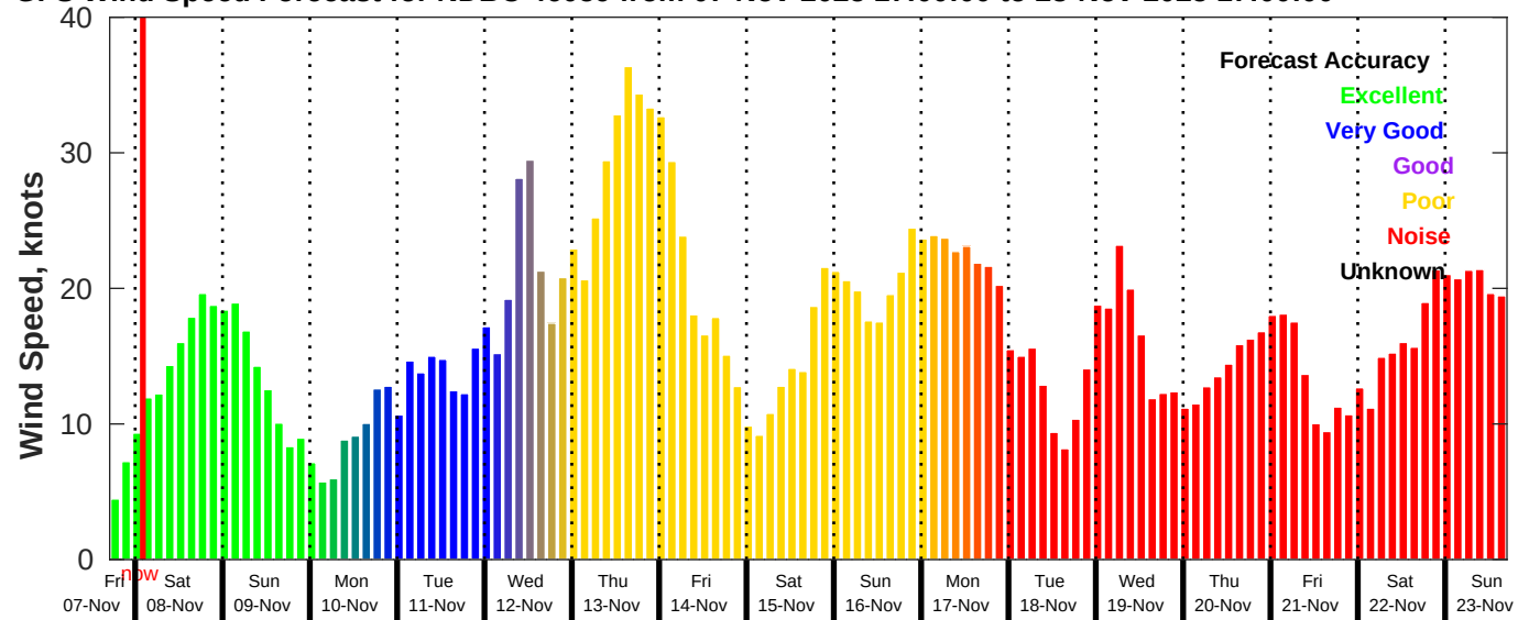
GFS Wind Speed Forecast for NDBC 46059 from 07-Nov-2025 17:00:00 to 23-Nov-2025 17:00:00
