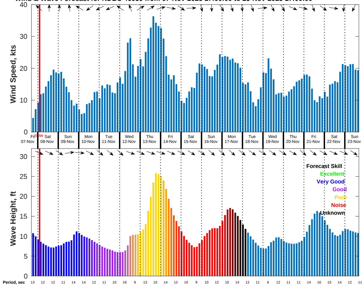
Wind & Wave Forecast for NDBC 46059 from 07-Nov-2025 17:00:00 to 23-Nov-2025 17:00:00
