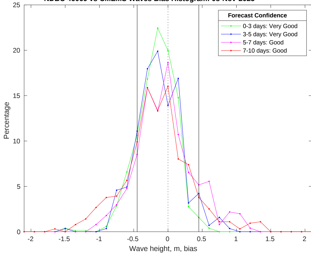
NDBC 46069 vs CMEMS Waves Bias Histogram: 08-Nov-2025
