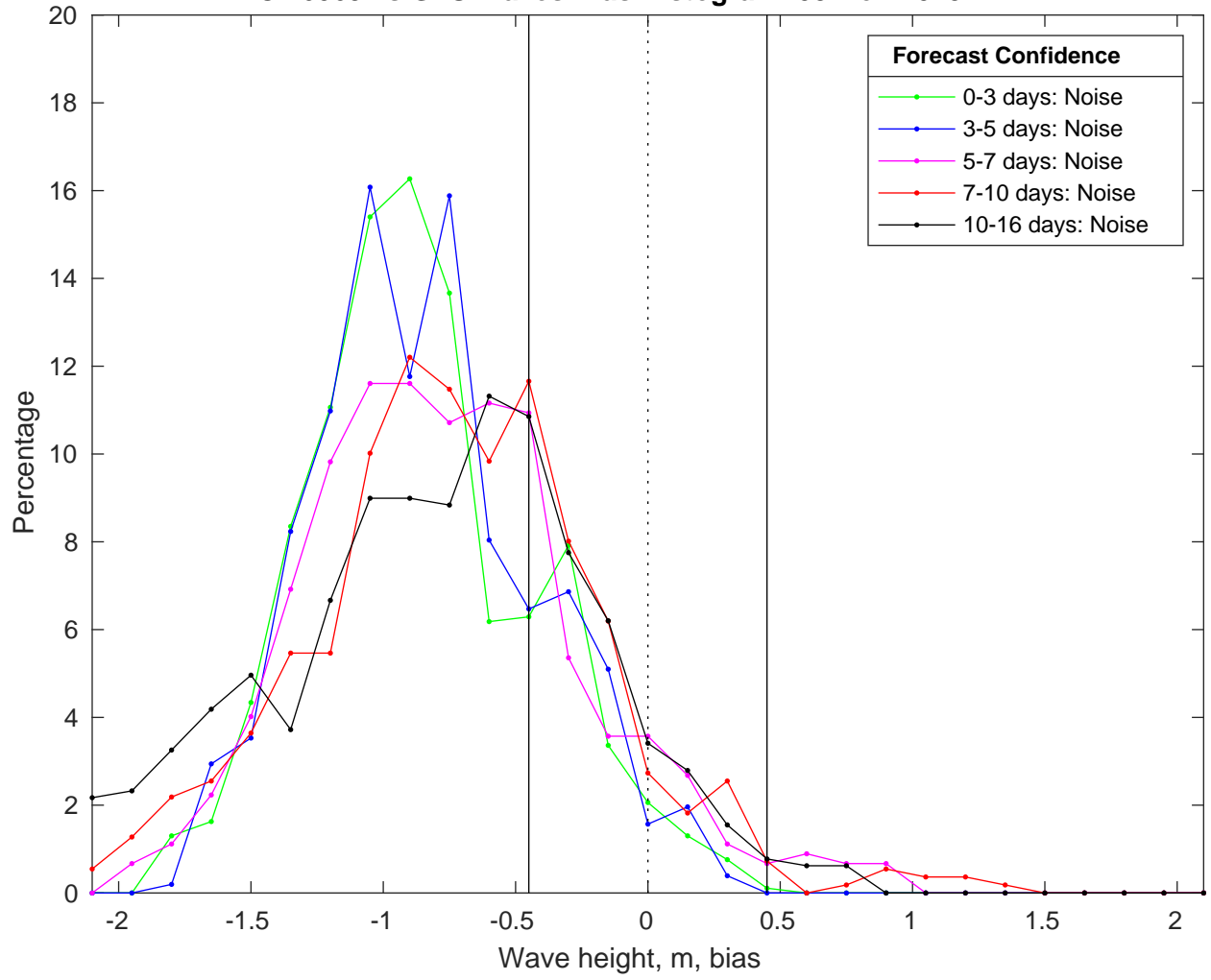
NDBC 46069 vs GFS Waves Bias Histogram: 08-Nov-2025
