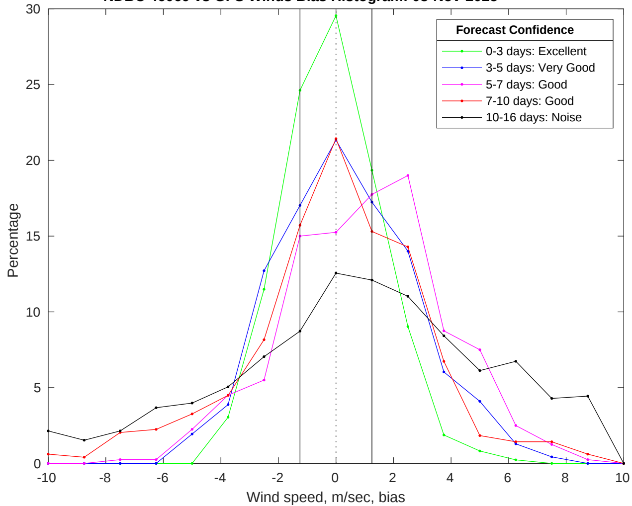
NDBC 46069 vs GFS Winds Bias Histogram: 08-Nov-2025
