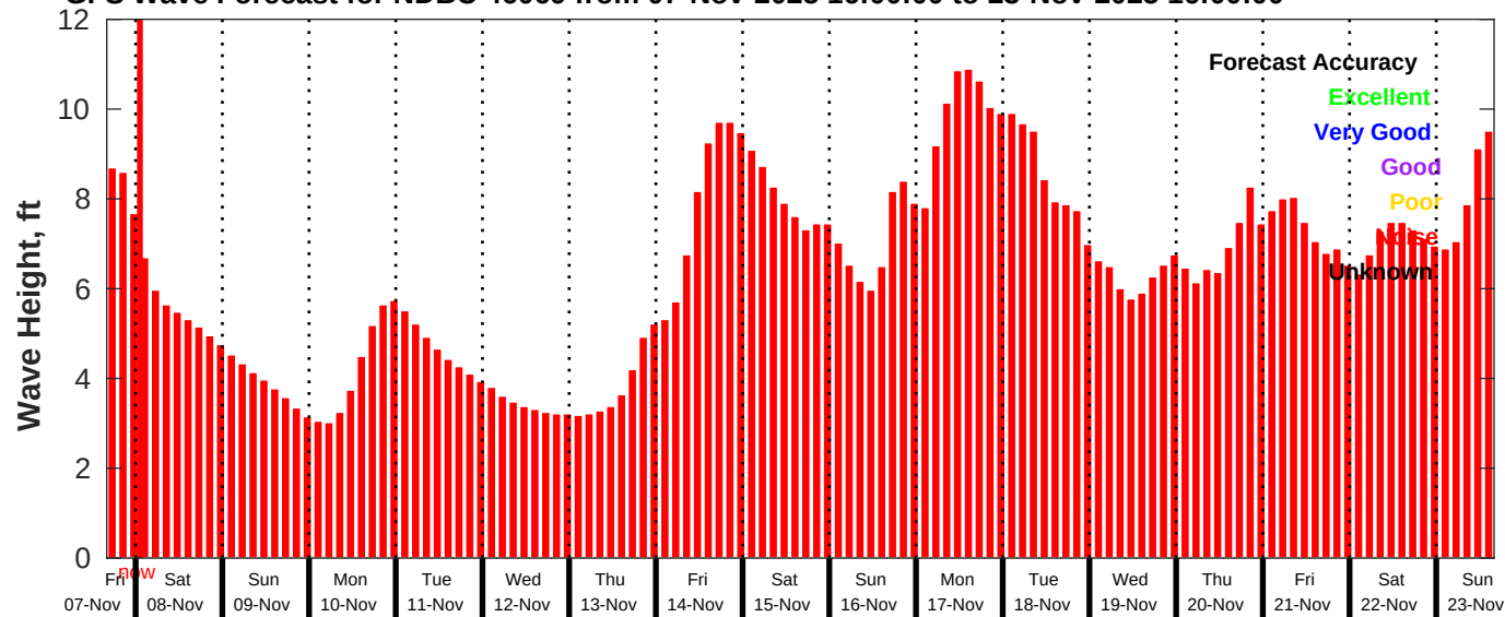
GFS Wave Forecast for NDBC 46069 from 07-Nov-2025 16:00:00 to 23-Nov-2025 16:00:00
