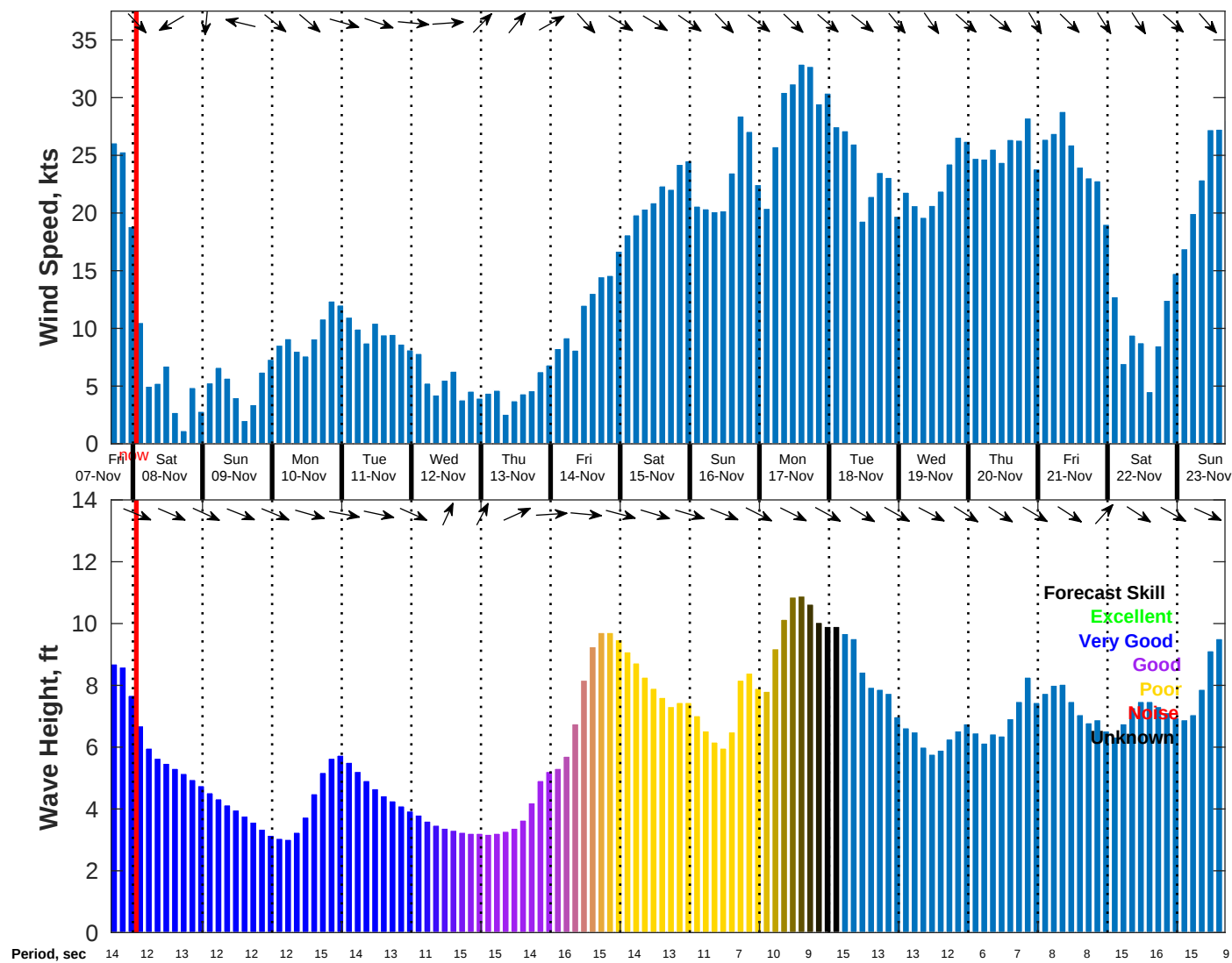
Wind & Wave Forecast for NDBC 46069 from 07-Nov-2025 16:00:00 to 23-Nov-2025 16:00:00
