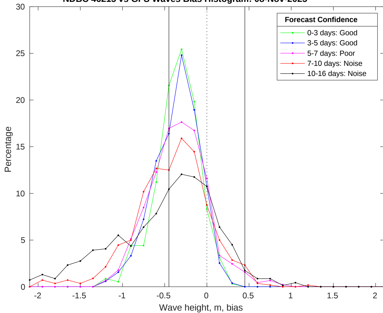
NDBC 46215 vs GFS Waves Bias Histogram: 08-Nov-2025
