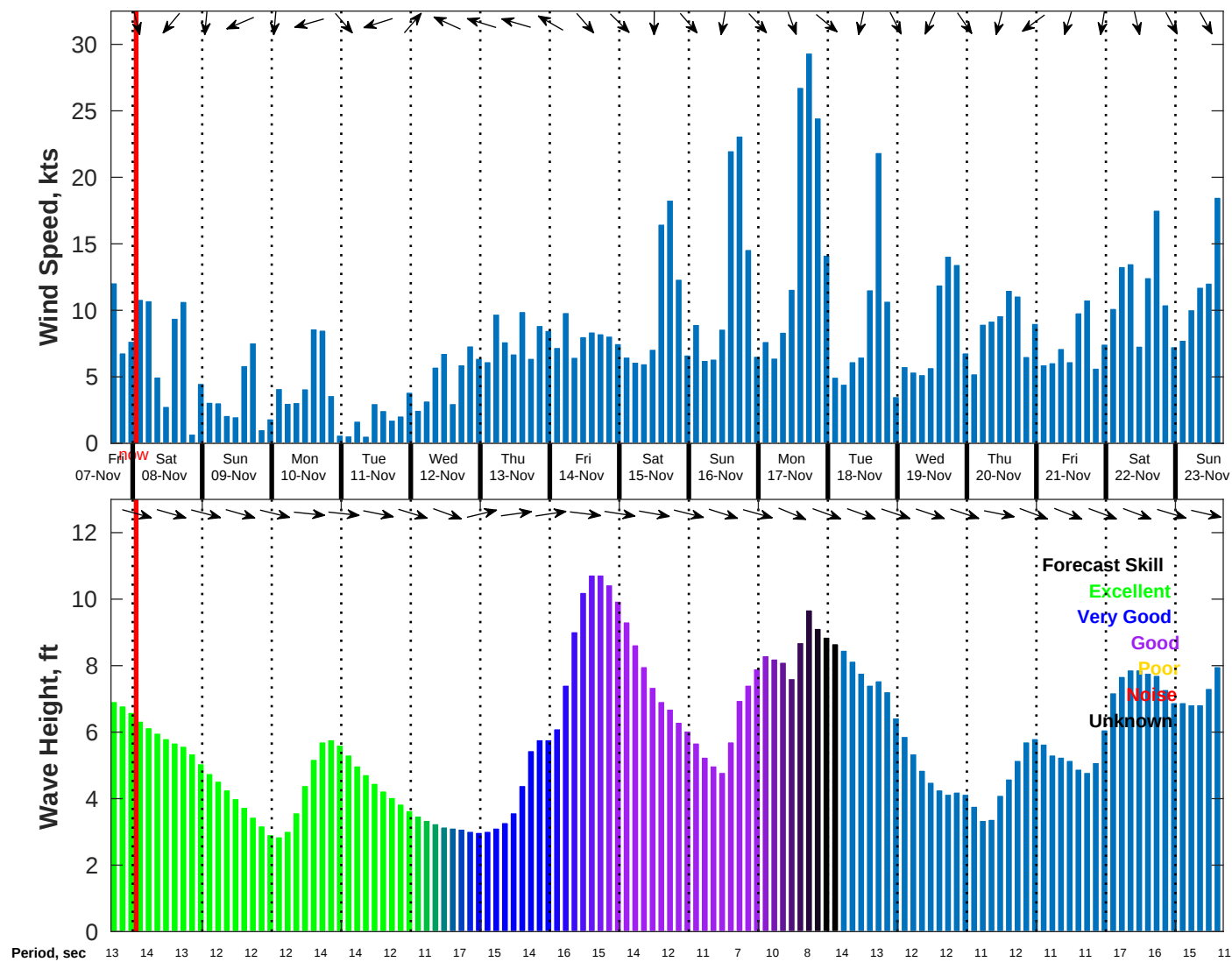
Wind & Wave Forecast for NDBC 46215 from 07-Nov-2025 16:00:00 to 23-Nov-2025 16:00:00
