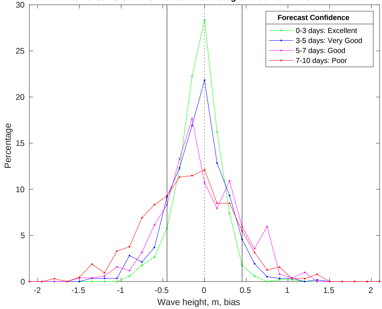
NDBC 46259 vs CMEMS Waves Bias Histogram: 08-Nov-2025
