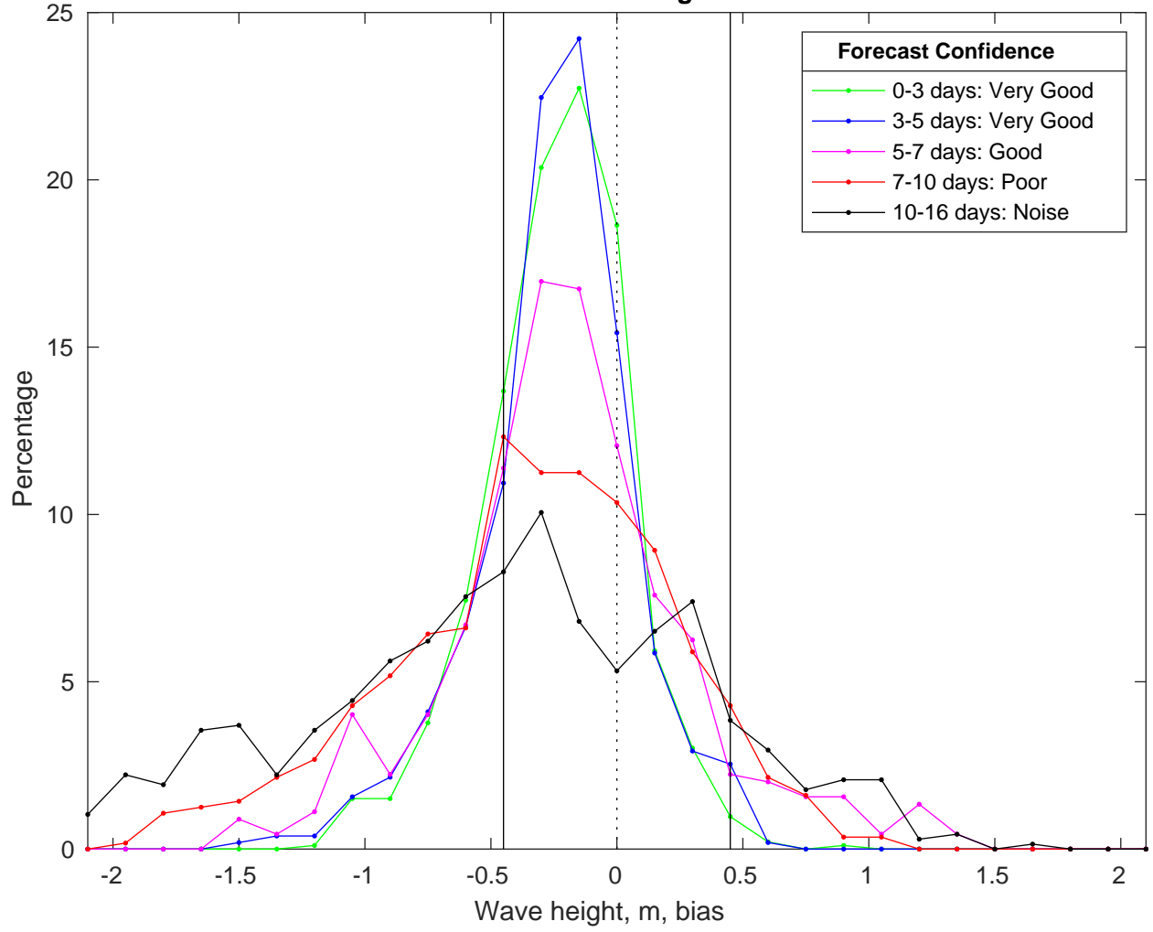
NDBC 46259 vs GFS Waves Bias Histogram: 08-Nov-2025
