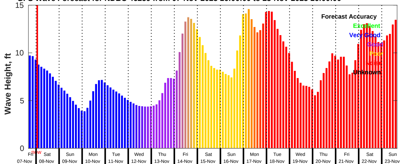
GFS Wave Forecast for NDBC 46259 from 07-Nov-2025 16:00:00 to 23-Nov-2025 16:00:00
