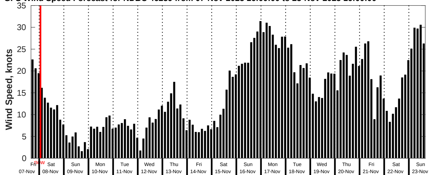
GFS Wind Speed Forecast for NDBC 46259 from 07-Nov-2025 16:00:00 to 23-Nov-2025 16:00:00
