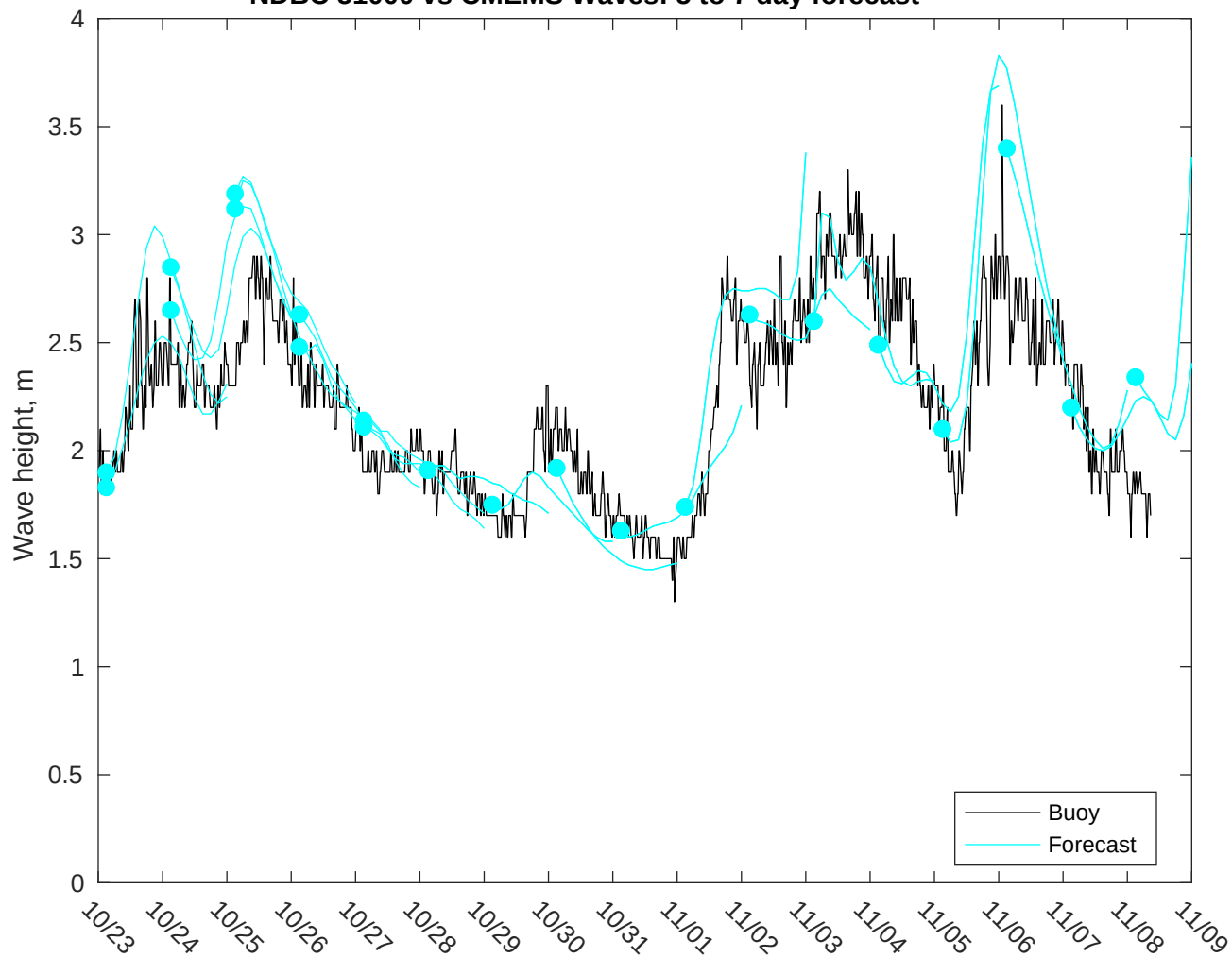
NDBC 51000 vs CMEMS Waves: 5 to 7 day forecast
