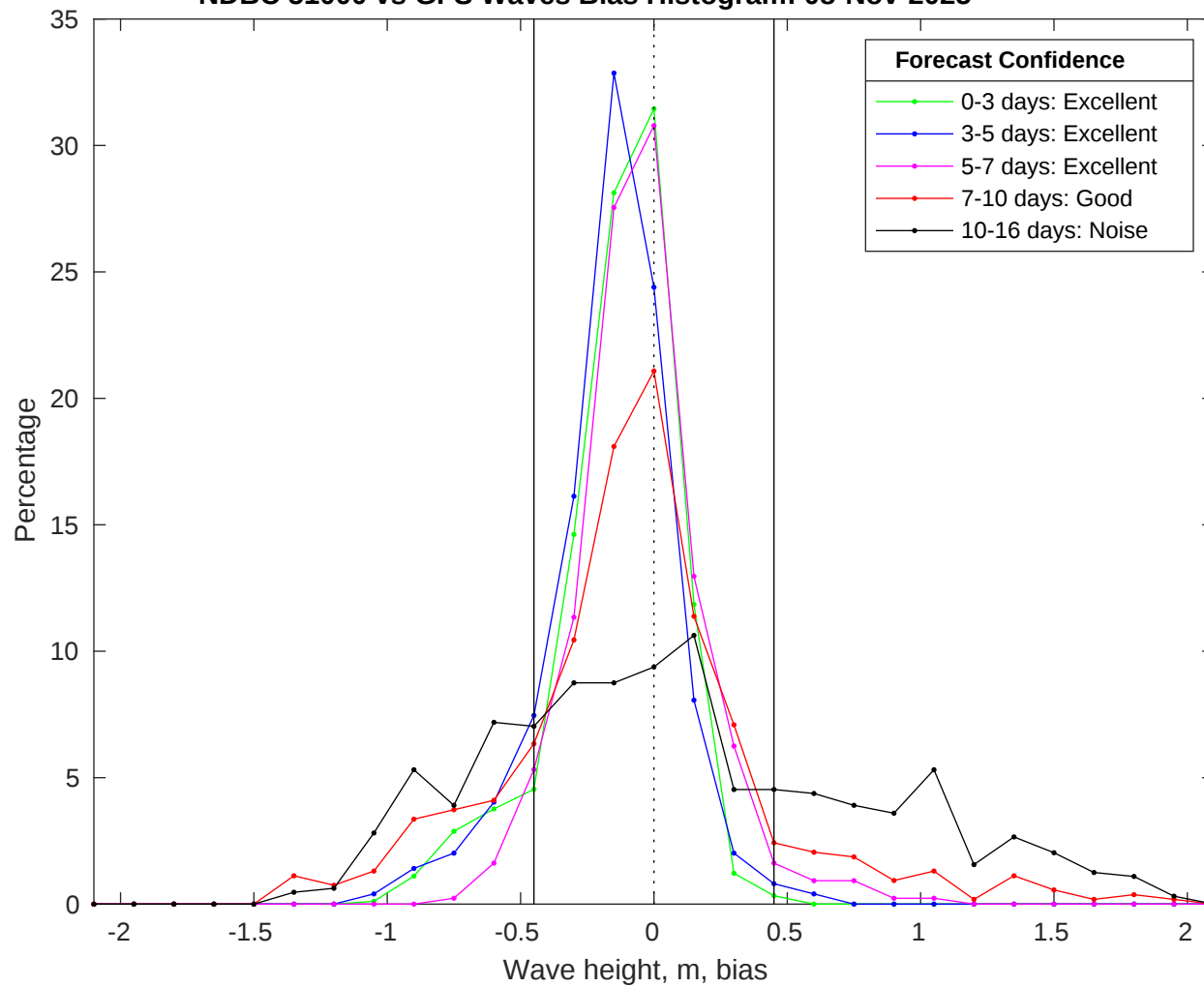
NDBC 51000 vs GFS Waves Bias Histogram: 08-Nov-2025
