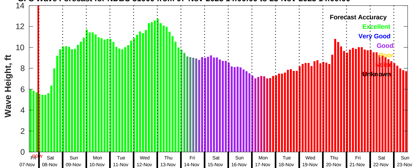
GFS Wave Forecast for NDBC 51000 from 07-Nov-2025 14:00:00 to 23-Nov-2025 14:00:00
