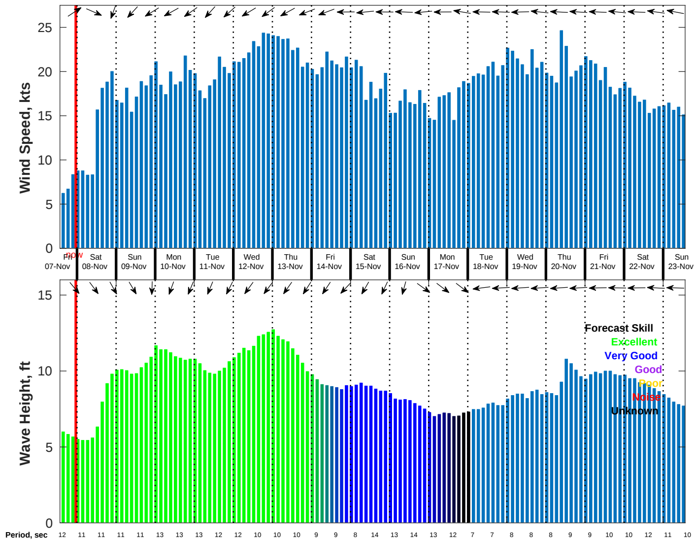
Wind & Wave Forecast for NDBC 51000 from 07-Nov-2025 14:00:00 to 23-Nov-2025 14:00:00
