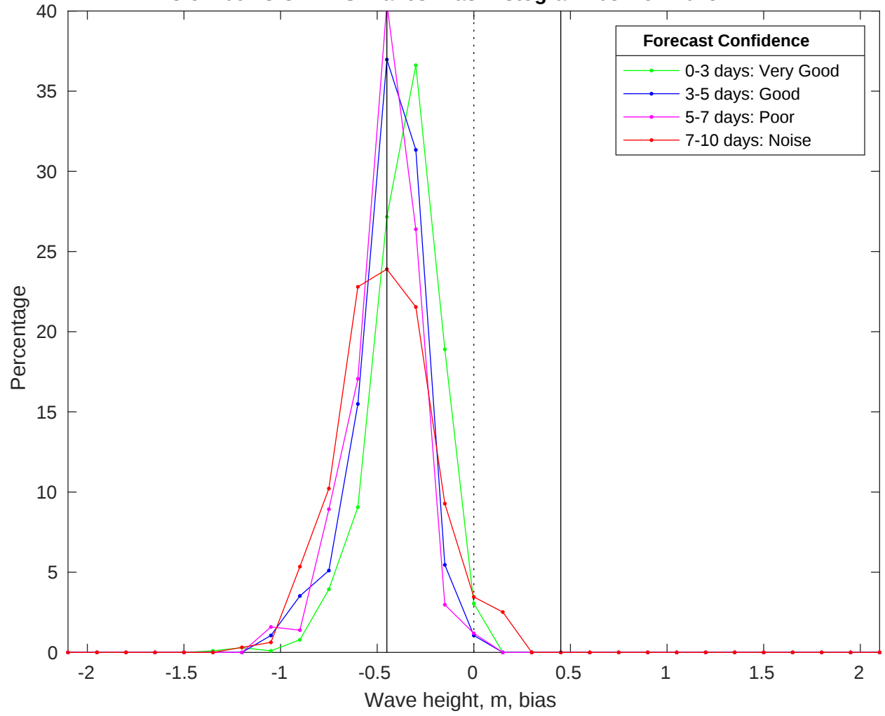
NDBC 51209 vs CMEMS Waves Bias Histogram: 08-Nov-2025
