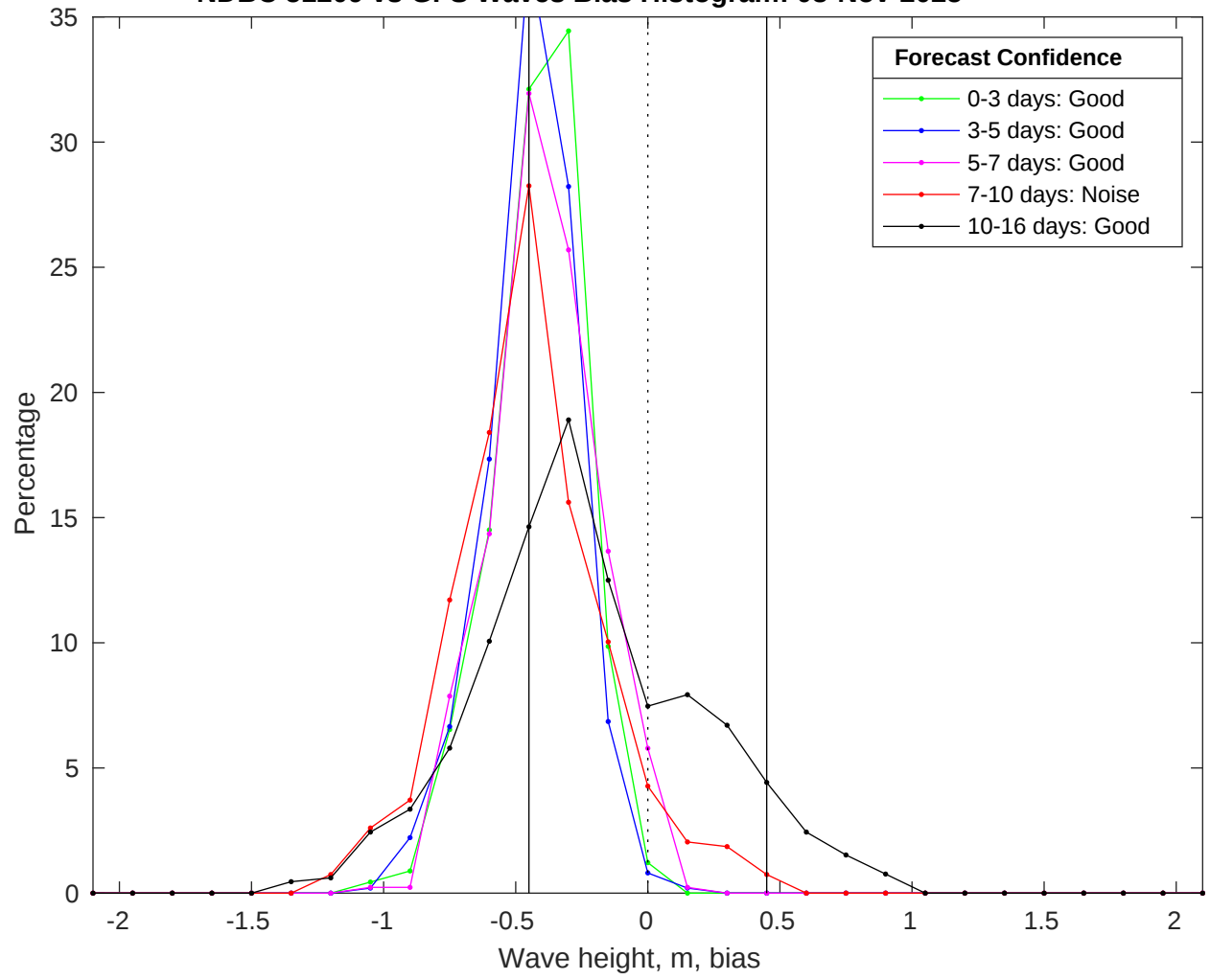
NDBC 51209 vs GFS Waves Bias Histogram: 08-Nov-2025
