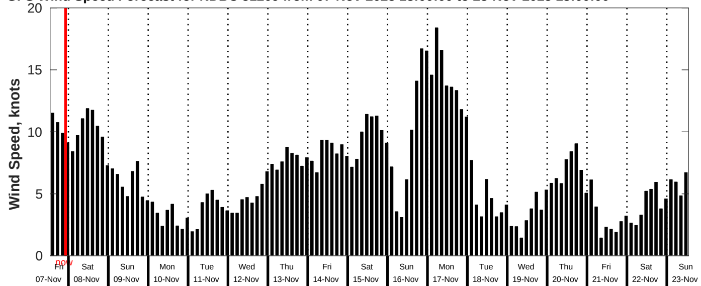
GFS Wind Speed Forecast for NDBC 51209 from 07-Nov-2025 13:00:00 to 23-Nov-2025 13:00:00
