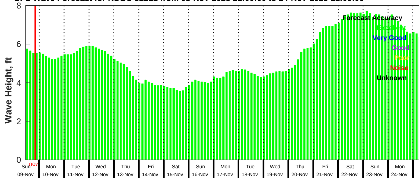
GFS Wave Forecast for NDBC 52211 from 08-Nov-2025 11:00:00 to 24-Nov-2025 11:00:00
