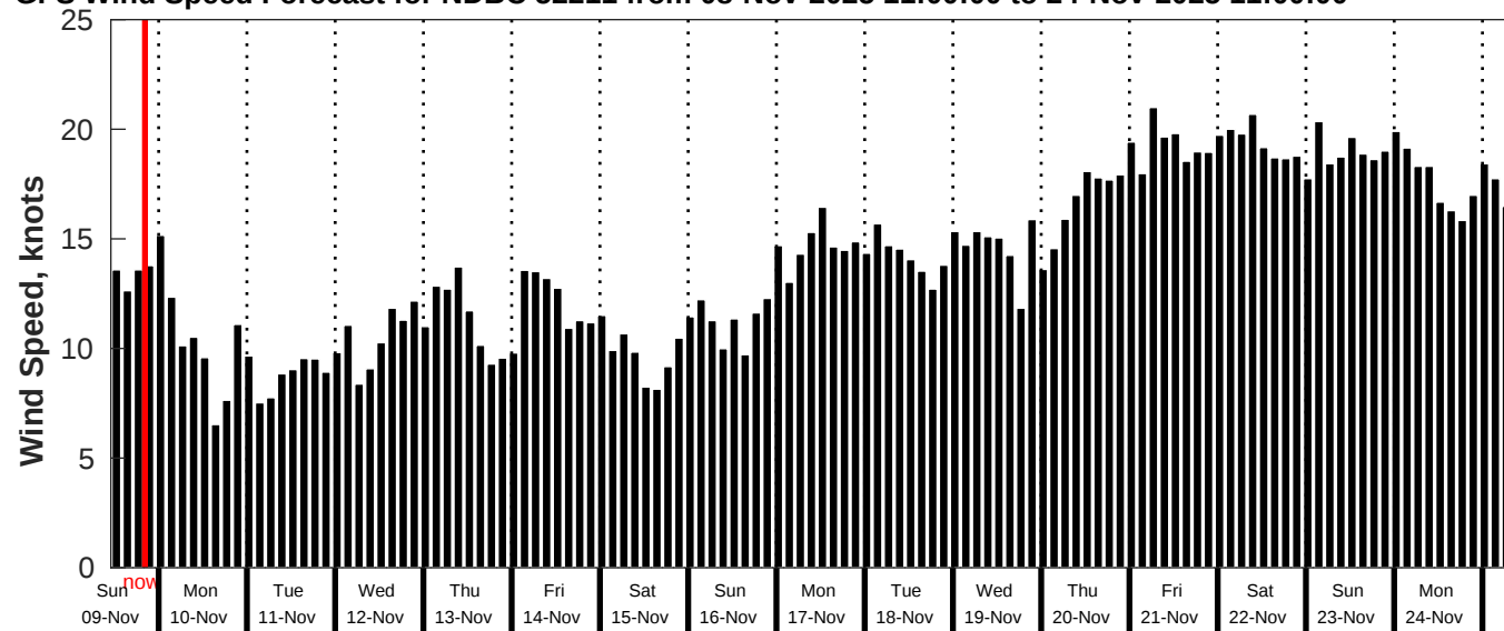
GFS Wind Speed Forecast for NDBC 52211 from 08-Nov-2025 11:00:00 to 24-Nov-2025 11:00:00
