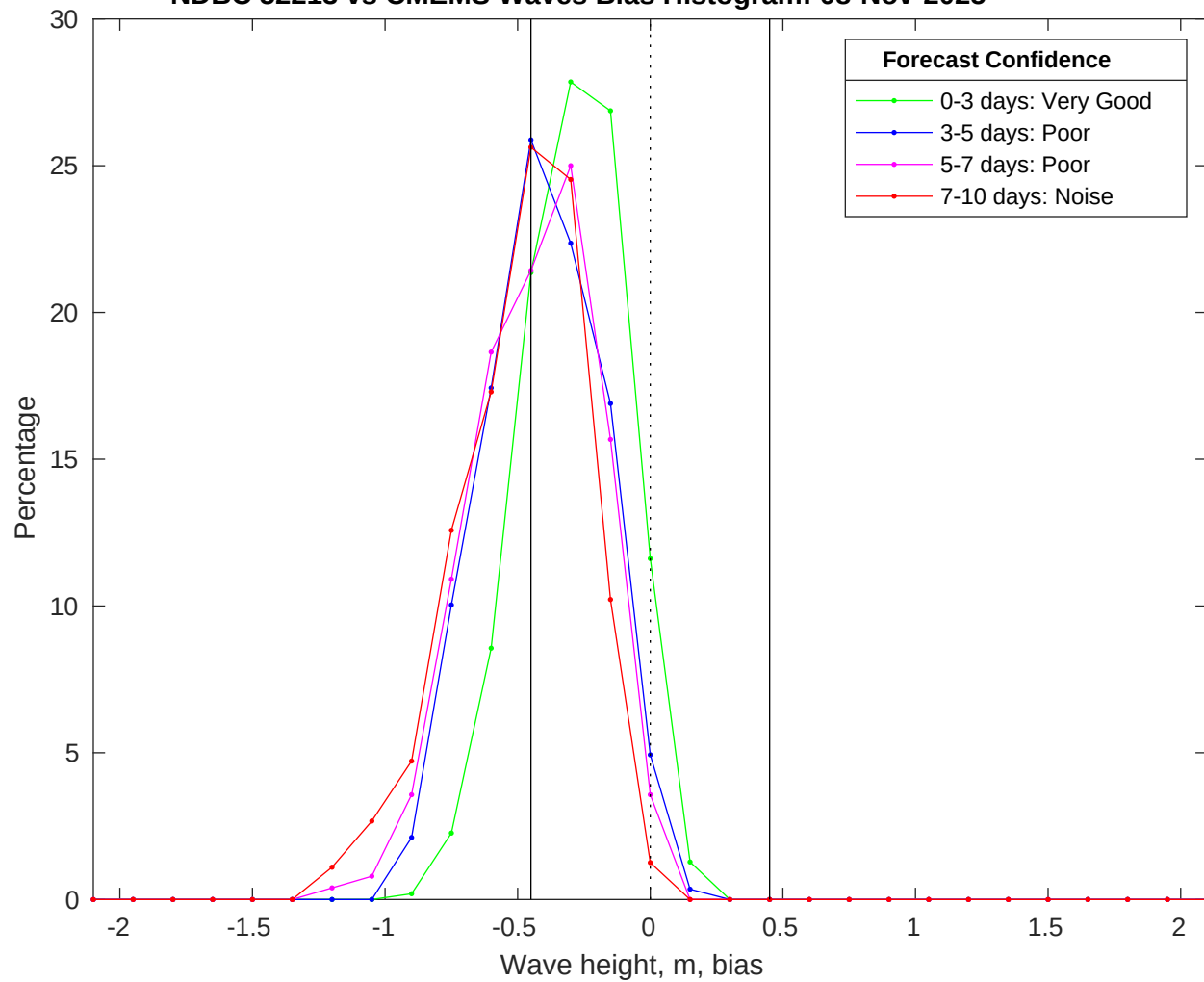
NDBC 52213 vs CMEMS Waves Bias Histogram: 08-Nov-2025
