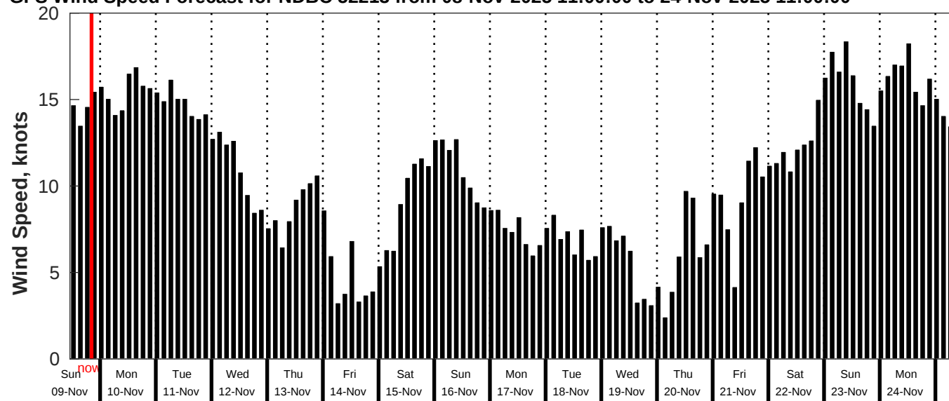
GFS Wind Speed Forecast for NDBC 52213 from 08-Nov-2025 11:00:00 to 24-Nov-2025 11:00:00
