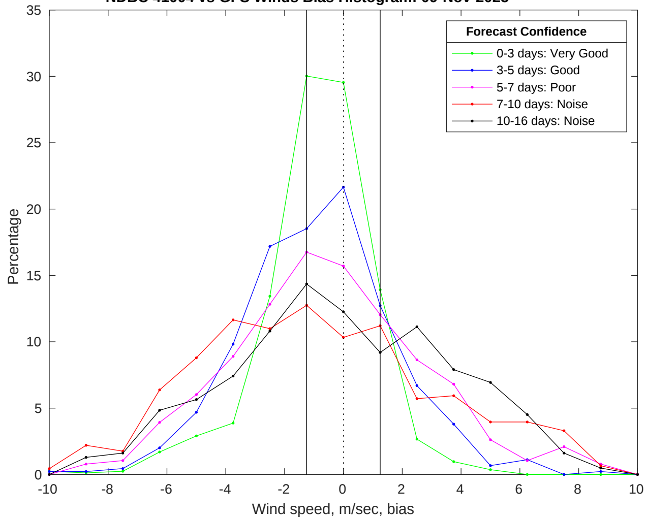
NDBC 41004 vs GFS Winds Bias Histogram: 09-Nov-2025
