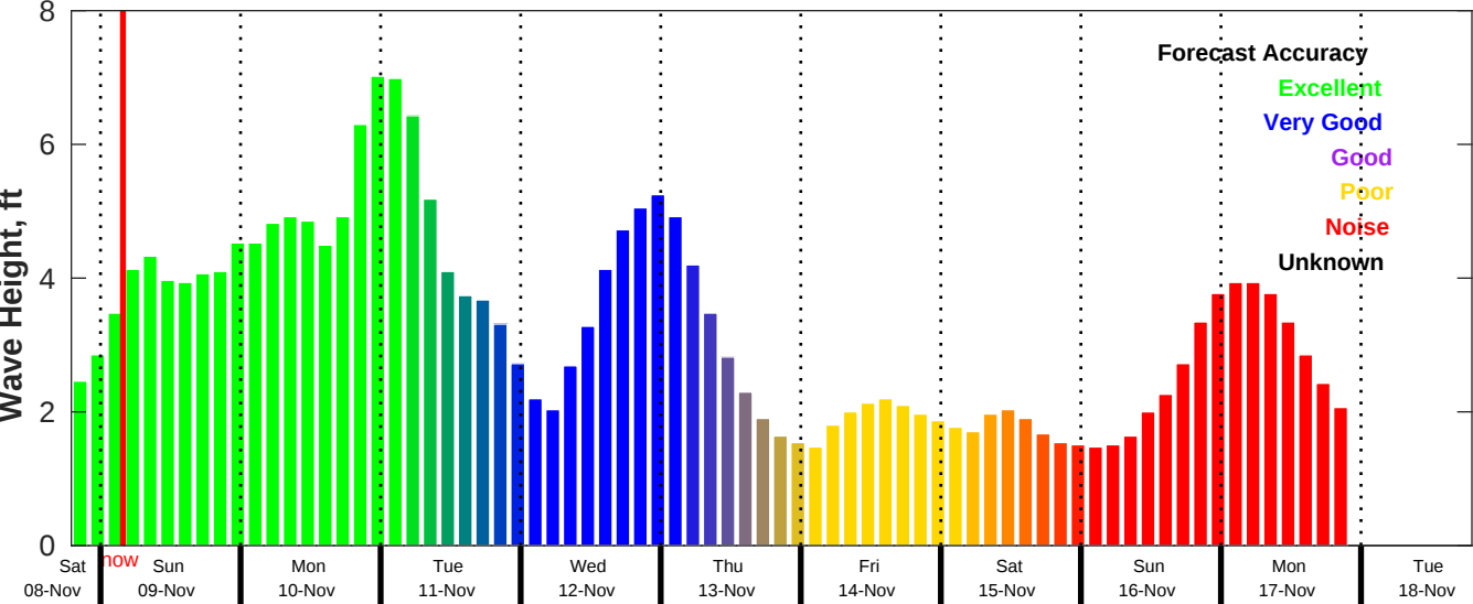
CMEMS Wave Forecast for NDBC 41004 from 08-Nov-2025 19:00:00 to 18-Nov-2025 19:00:00
