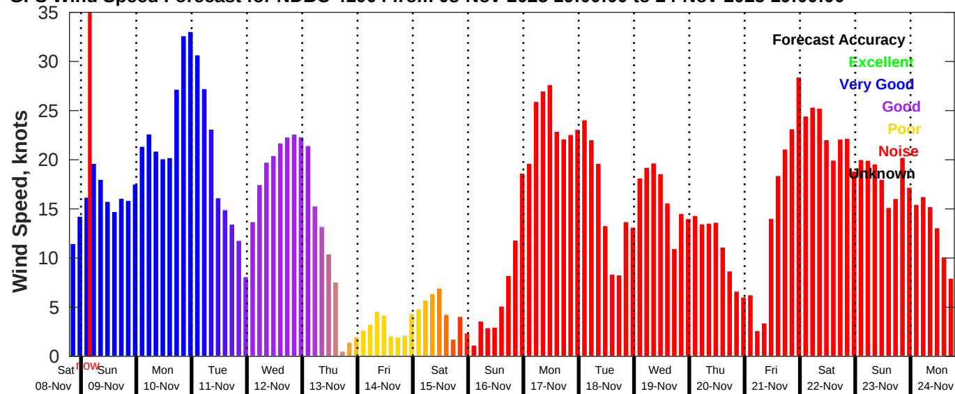
GFS Wind Speed Forecast for NDBC 41004 from 08-Nov-2025 19:00:00 to 24-Nov-2025 19:00:00
