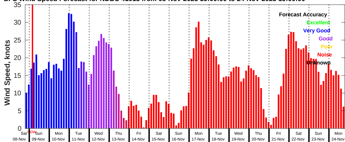
GFS Wind Speed Forecast for NDBC 41013 from 08-Nov-2025 19:00:00 to 24-Nov-2025 19:00:00
