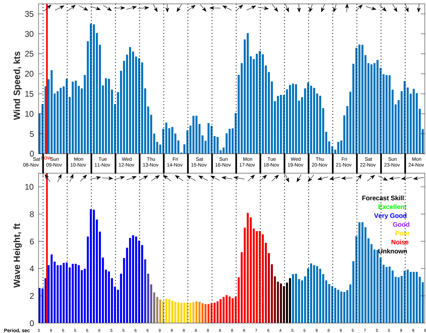
Wind & Wave Forecast for NDBC 41013 from 08-Nov-2025 19:00:00 to 24-Nov-2025 19:00:00
