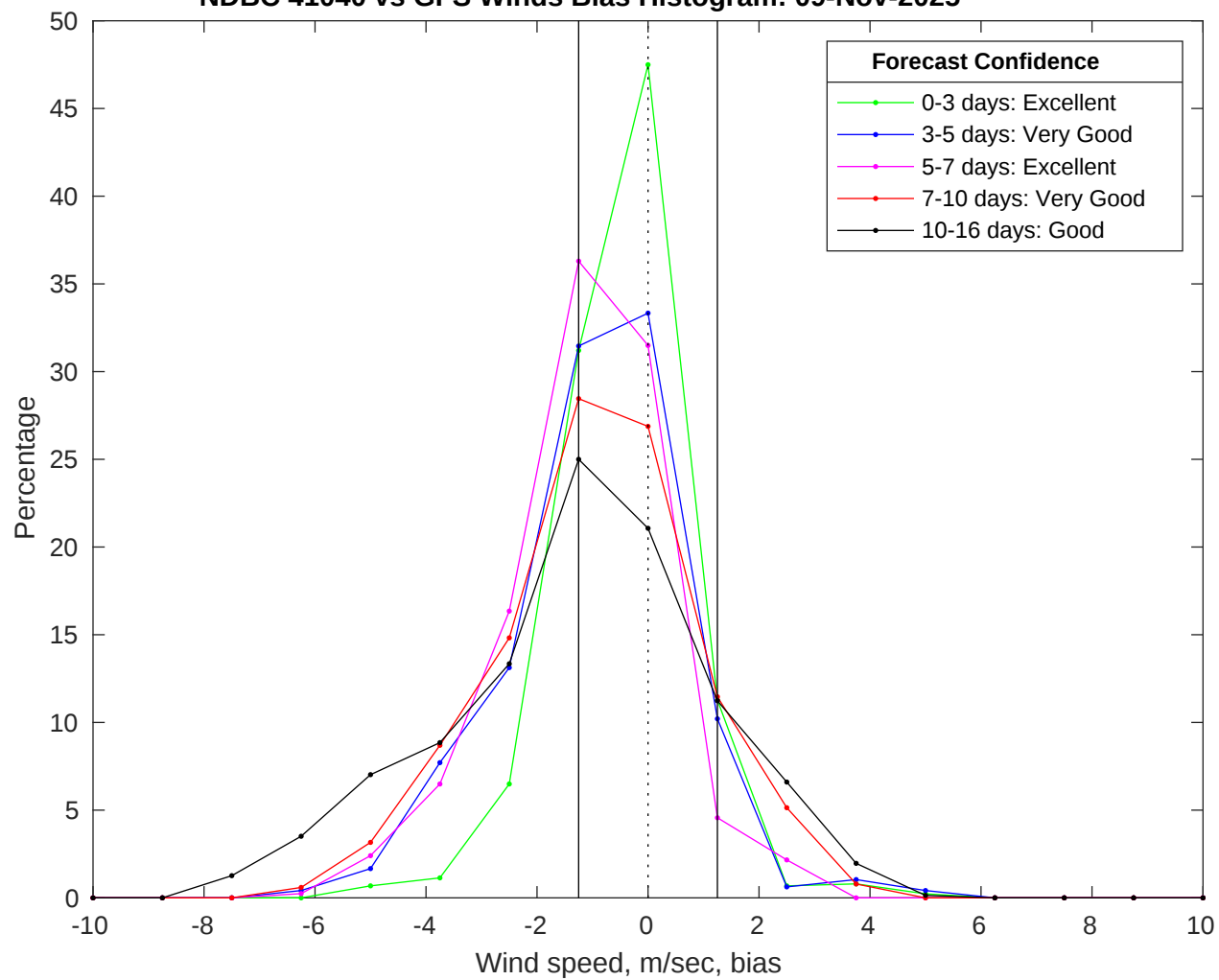
NDBC 41040 vs GFS Winds Bias Histogram: 09-Nov-2025
