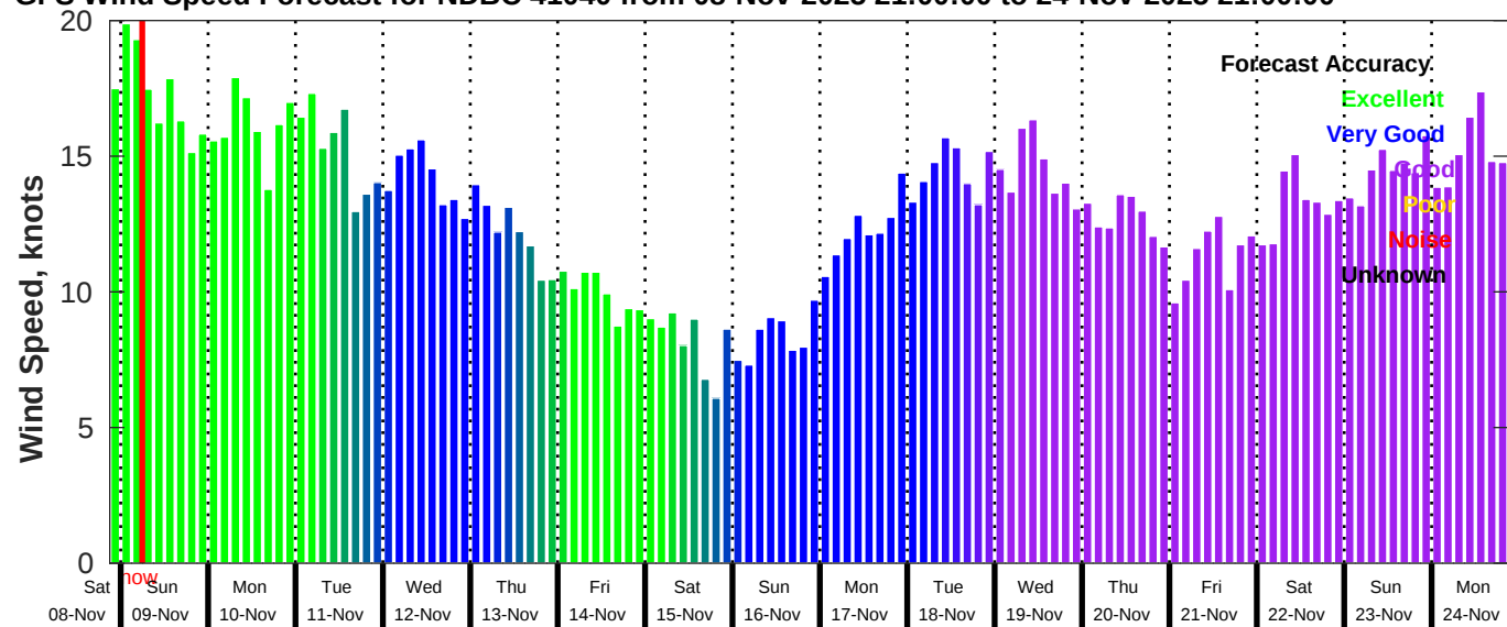
GFS Wind Speed Forecast for NDBC 41040 from 08-Nov-2025 21:00:00 to 24-Nov-2025 21:00:00
