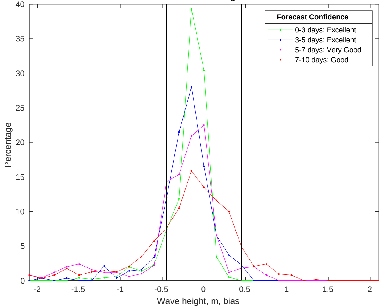
NDBC 42019 vs CMEMS Waves Bias Histogram: 09-Nov-2025
