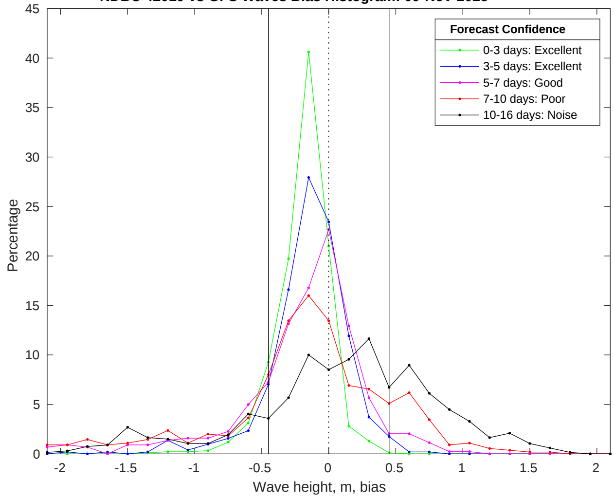
NDBC 42019 vs GFS Waves Bias Histogram: 09-Nov-2025
