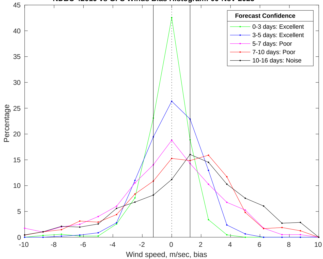
NDBC 42019 vs GFS Winds Bias Histogram: 09-Nov-2025
