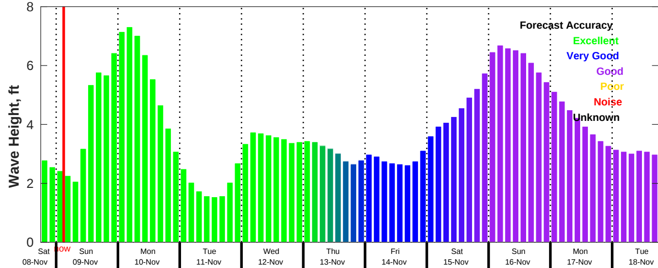
CMEMS Wave Forecast for NDBC 42019 from 08-Nov-2025 18:00:00 to 18-Nov-2025 18:00:00
