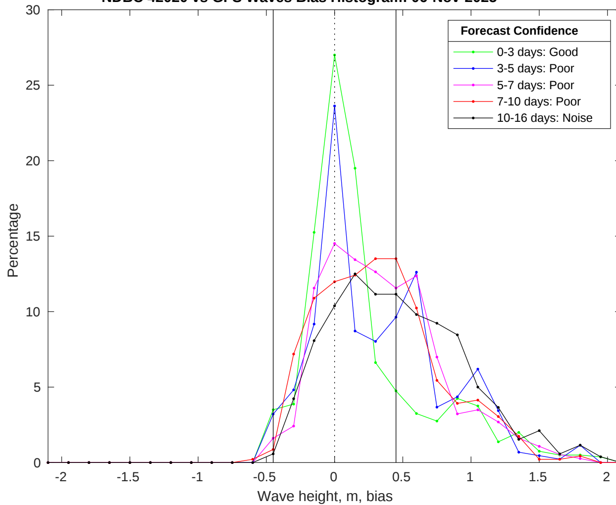
NDBC 42020 vs GFS Waves Bias Histogram: 06-Nov-2025
