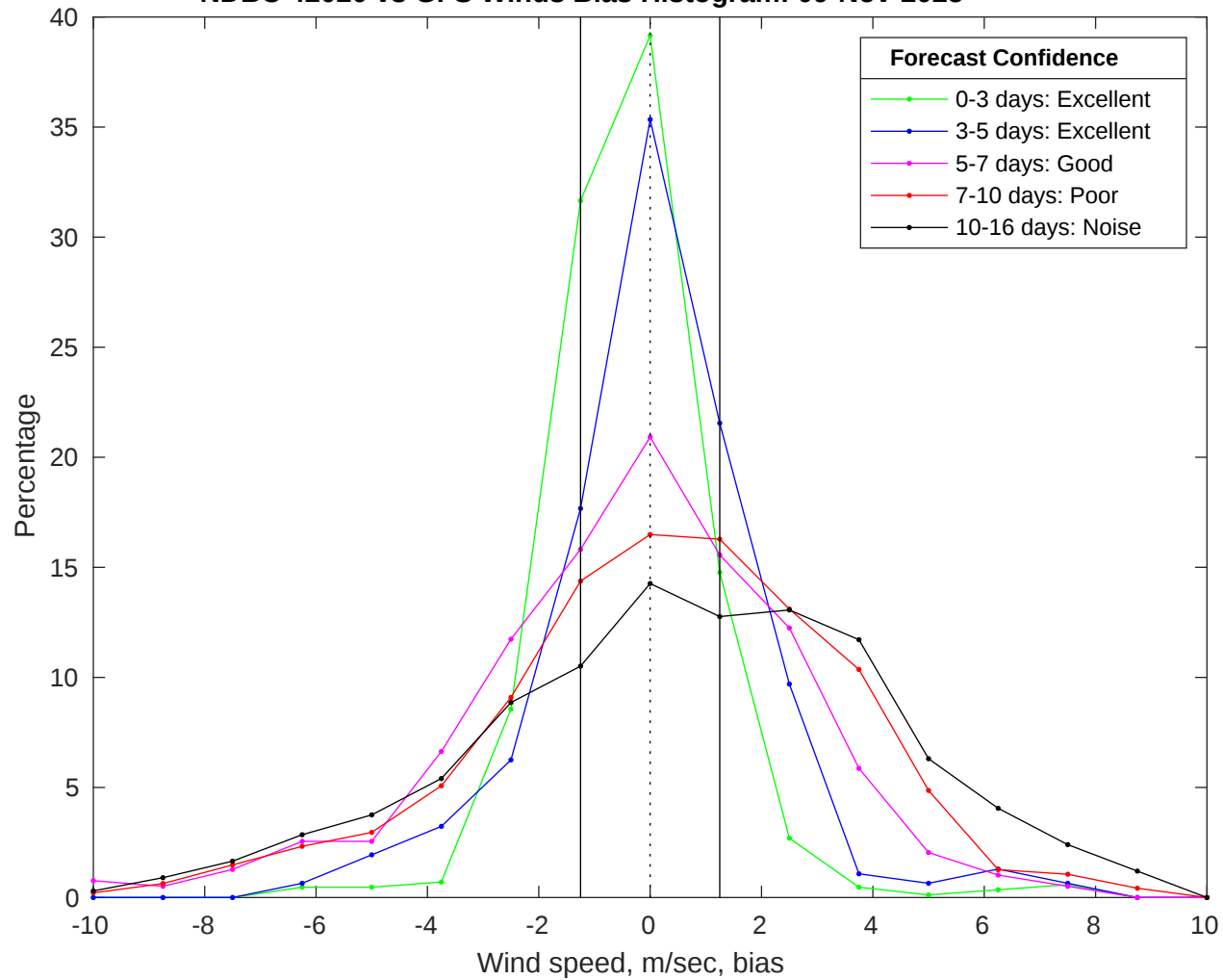
NDBC 42020 vs GFS Winds Bias Histogram: 09-Nov-2025
