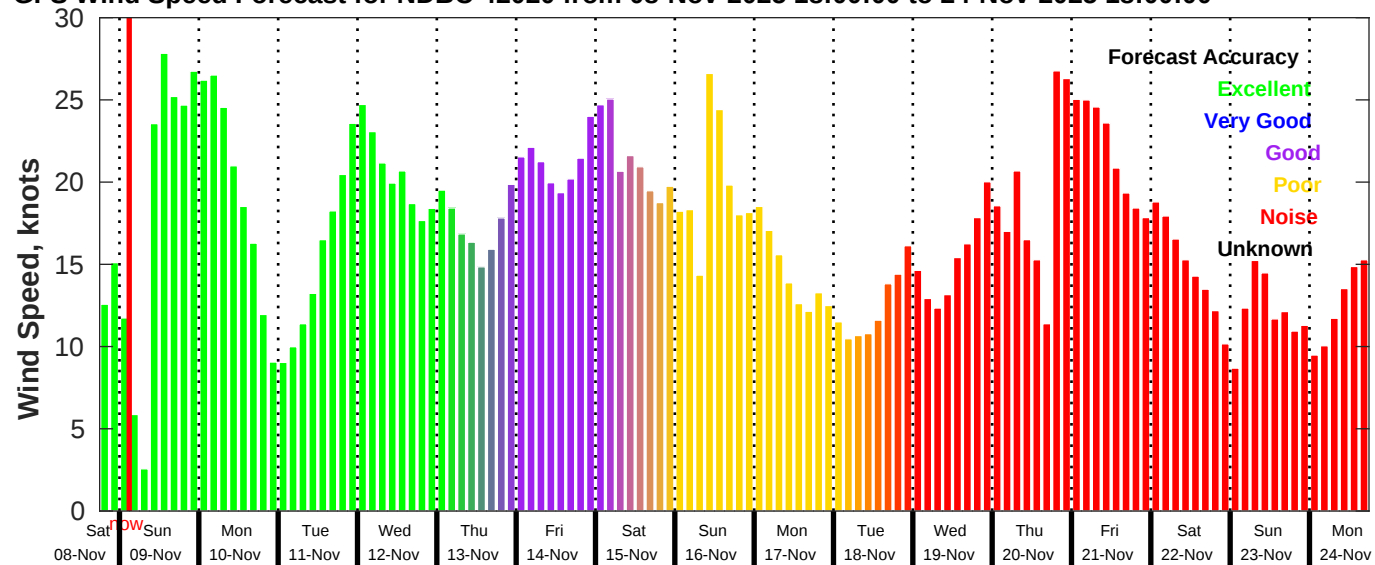
GFS Wind Speed Forecast for NDBC 42020 from 08-Nov-2025 18:00:00 to 24-Nov-2025 18:00:00
